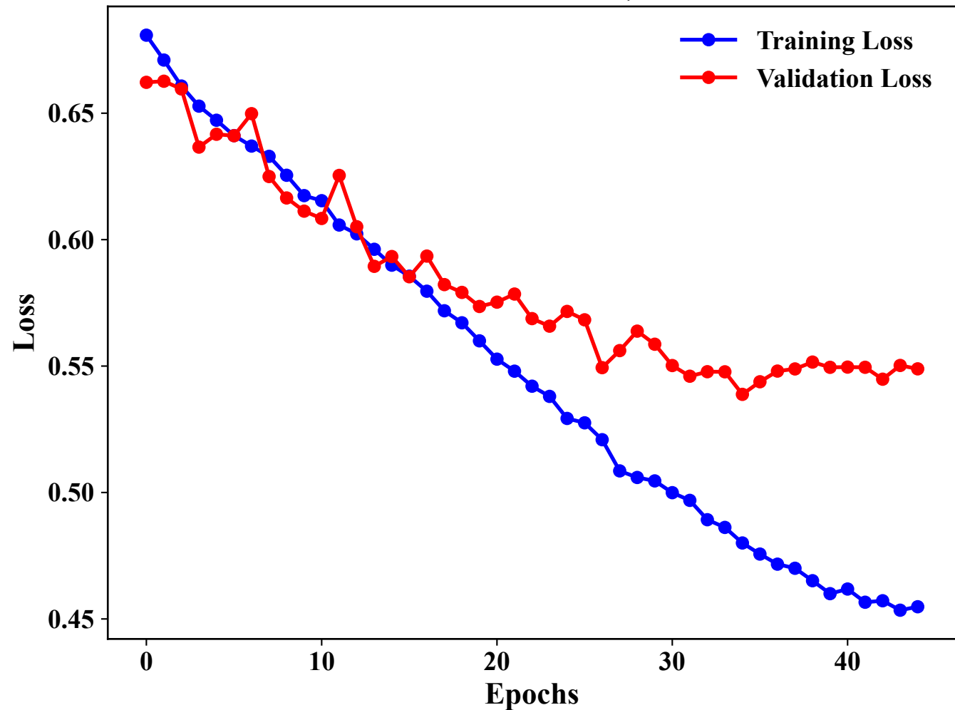
Loss Curves: Seed 16, Rank 3
